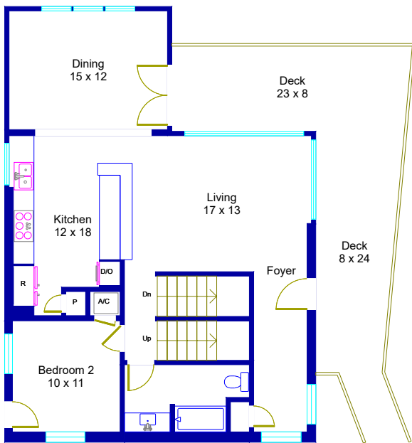
Main House Third Floor
